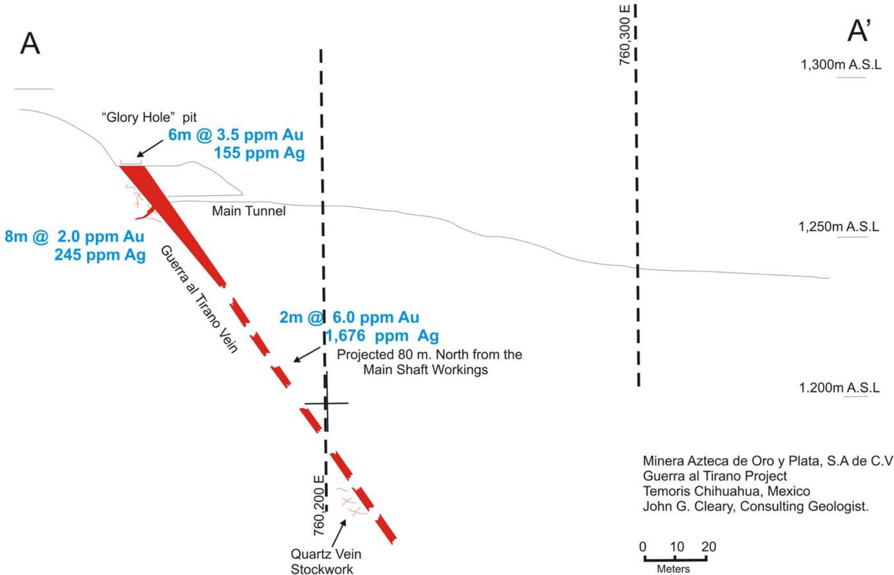
Figure 6. Guerra al Tirano Vein Cross Section A - A'
